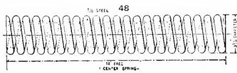
Fig. 1402. Long Center-spring
